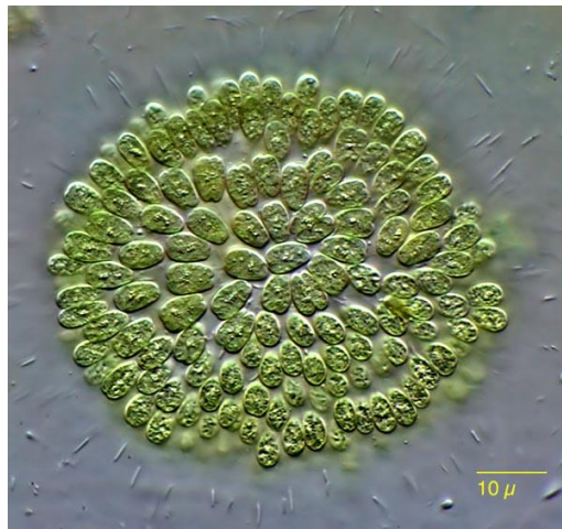
Coelosphaerium
